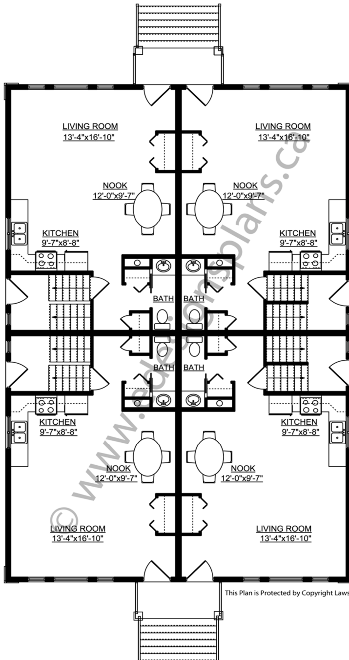
Main Floor
